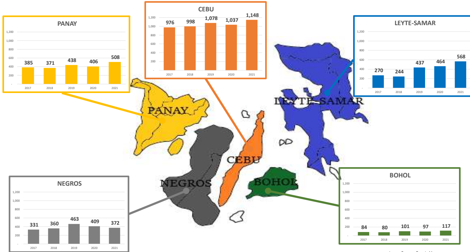
Five-year Non-Coincidental System Peak Demand (MW), 2017-2021
